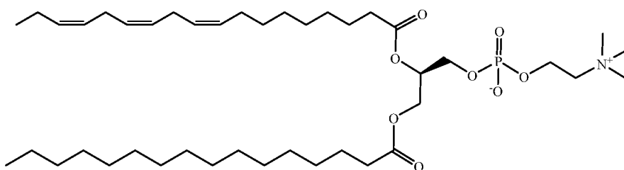
(R)-2-(((9Z, 12Z, 15Z)-octadeca-9, 12, 15-trienoyl)oxy)-3-((Z)-hexadec-9-enoyl)oxypropyl (2-(trimethylammonio)ethyl) phosphate ("MPC3")
